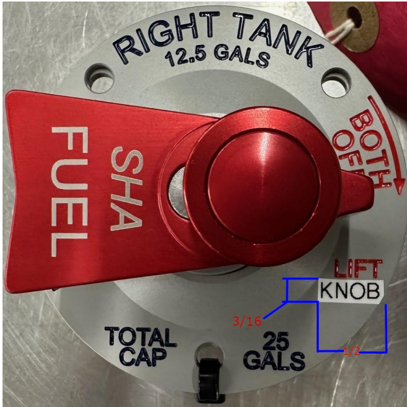
Figure 3 - Decal Installation and Dimensions as shown.
